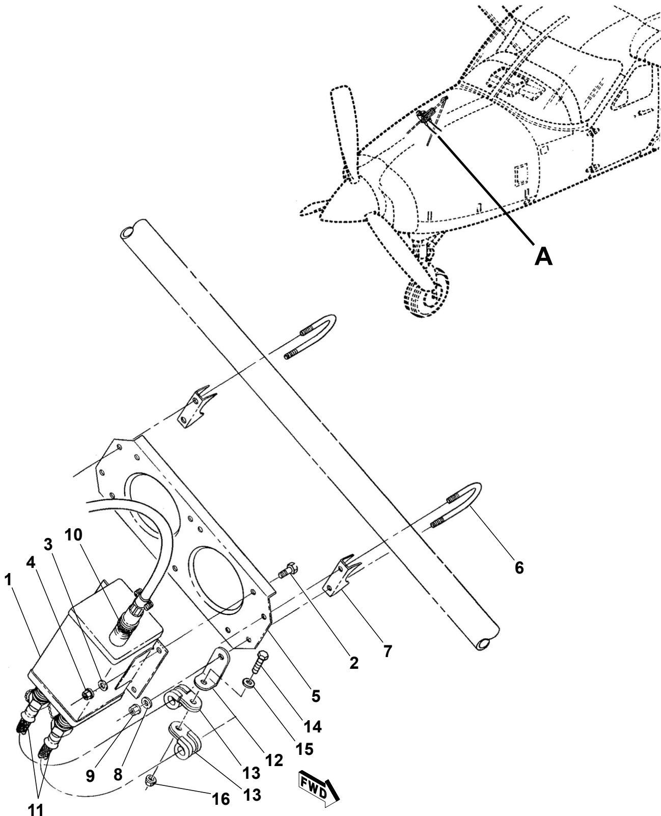
IGNITION EXCITER INSTALLATION Figure 01. (Sheet 1)
